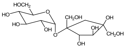
Sucrose; glucose and fructose
