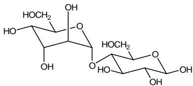
altose and glucose
