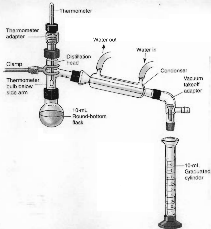
Apparatus for simple distillation.
