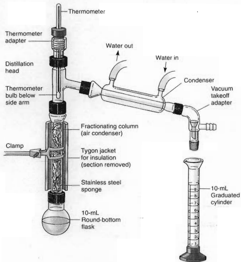
Apparatus for fractional distillation.
